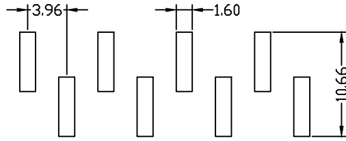
Type A PCB LAYOUT
