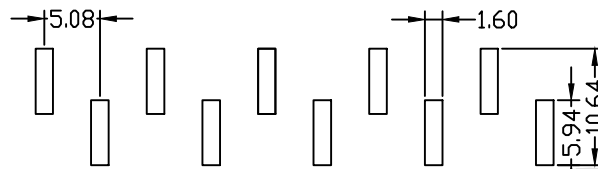
TYPE A PCB LAYOUT
