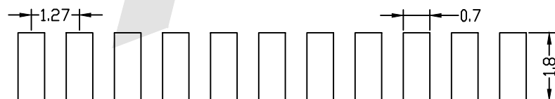
PCB LAYOUT
