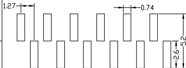
TYPE A PCB LAYOUT
