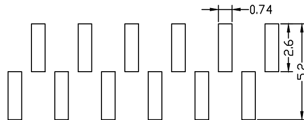
TYPE B PCB LAYOUT
