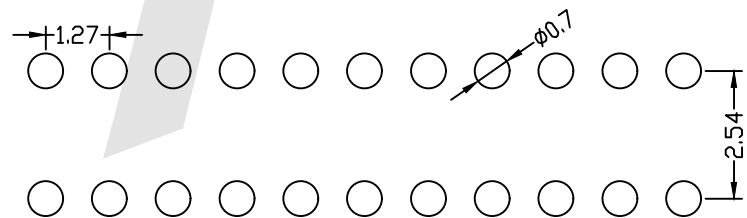
P. C. B LAYOUT
