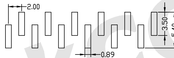
TYPE B PCB LAYOUT
