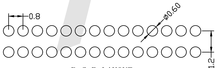
P. C. B LAYOUT
