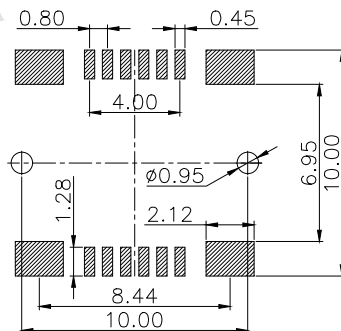
Recommended P.C.Board Layout (Tolerance:±0.05)
