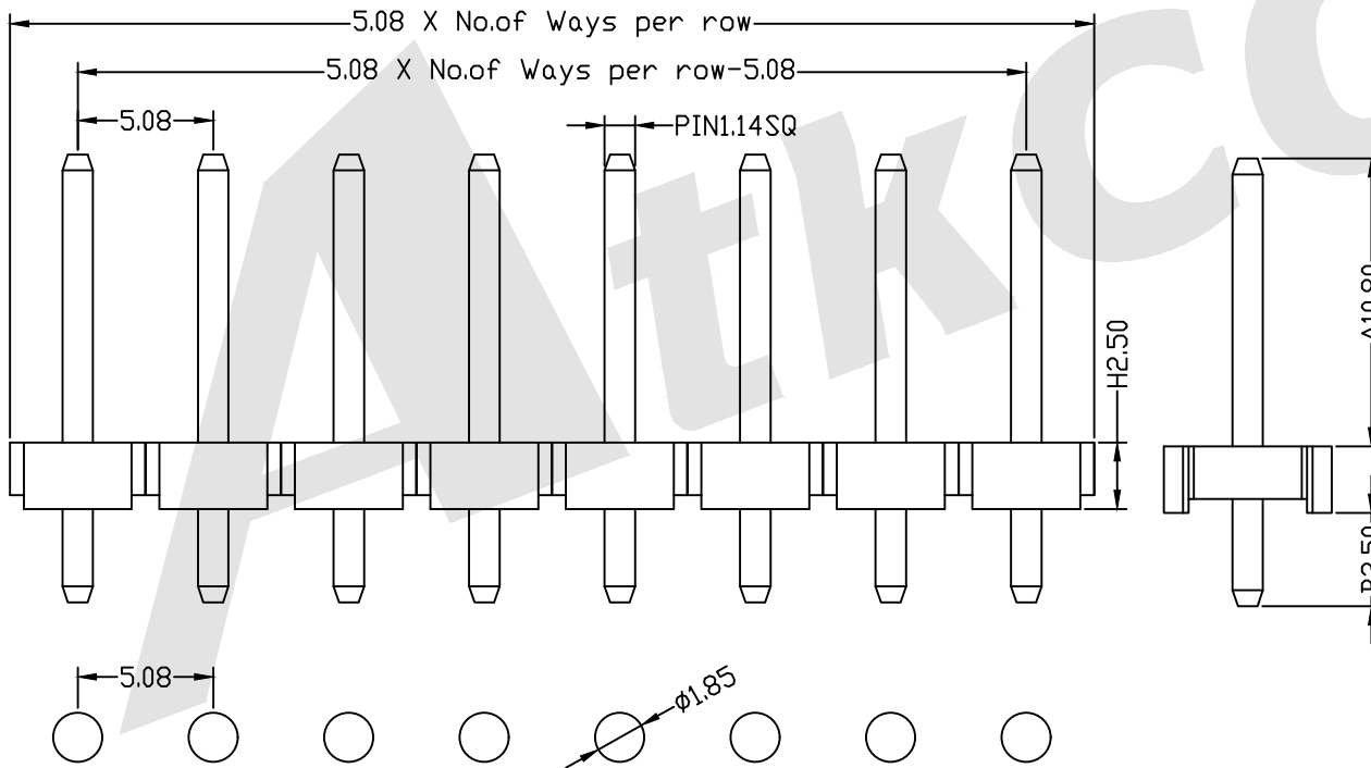
PCB LAYOUT
