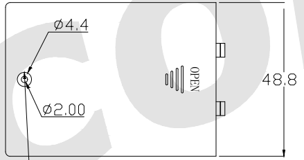
FORSELF-TAPPING SCREW
