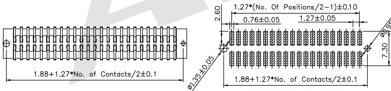
RECOMMENDED PCB LAYOUT (Tolerance: ±0.05)
