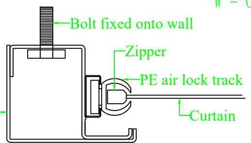
Side track-zipper air tight design
