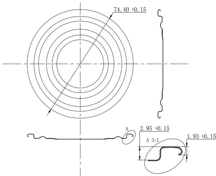
产品图Product Drawing
