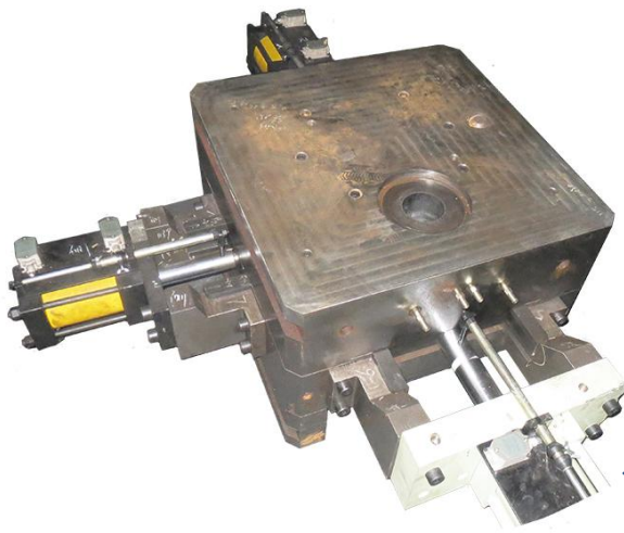
LED Light Heat Sink Aluminum Die Casting Mould LED灯壳散热器压铸模具
