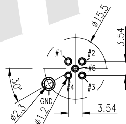
3~5P RECOMMENDED PCB LAYOUT; TOL: ±0.05mm
