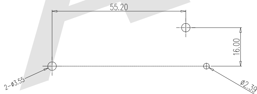
PCB LAYOUT
