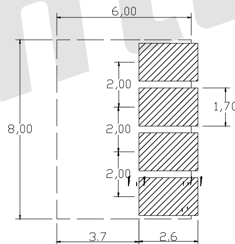
RECOMMENDED PCB LAYOUT TOP VIEW (. XX ± 0.05)
