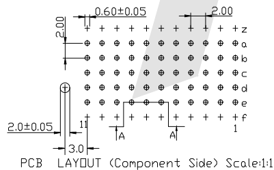
PCB LAYOUT (Component Side) Scale:1:1
