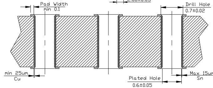
RECOMMENDED HOLE SPECIFICATIONS SECTION A-A SCALE 20:1
