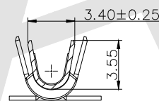
SECTION K-K 14-16awg
