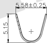
SECTION J-J
