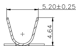
SECTION L-L
