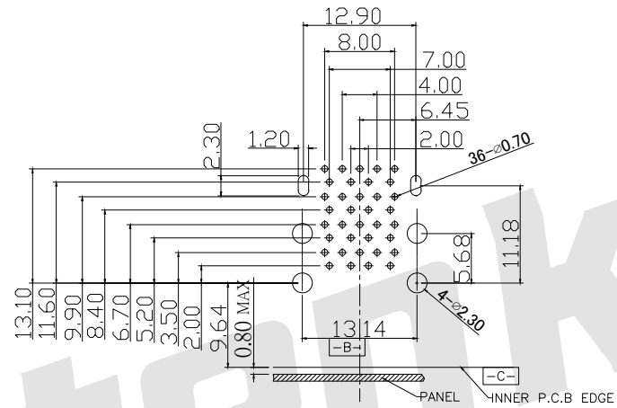
RECOMMENDED P.C.B. LAYOUT (1) (THICKNESS=1.6mm) (GENERAL TOLERANCE: ±0.05)
