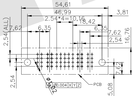
P. C. Body Hole Layout
