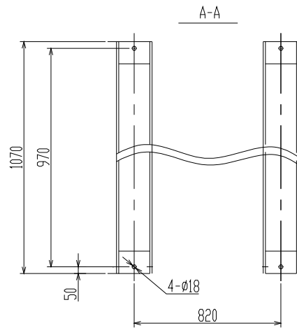
Base structure
