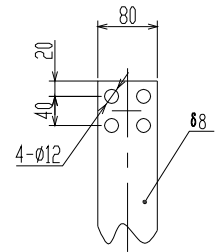
LV terminal
