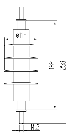
Surge arrester: HY5WS-17/50
