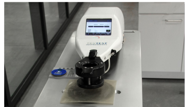
通气度试验台 Filter Material Air Permeability Test Platform
