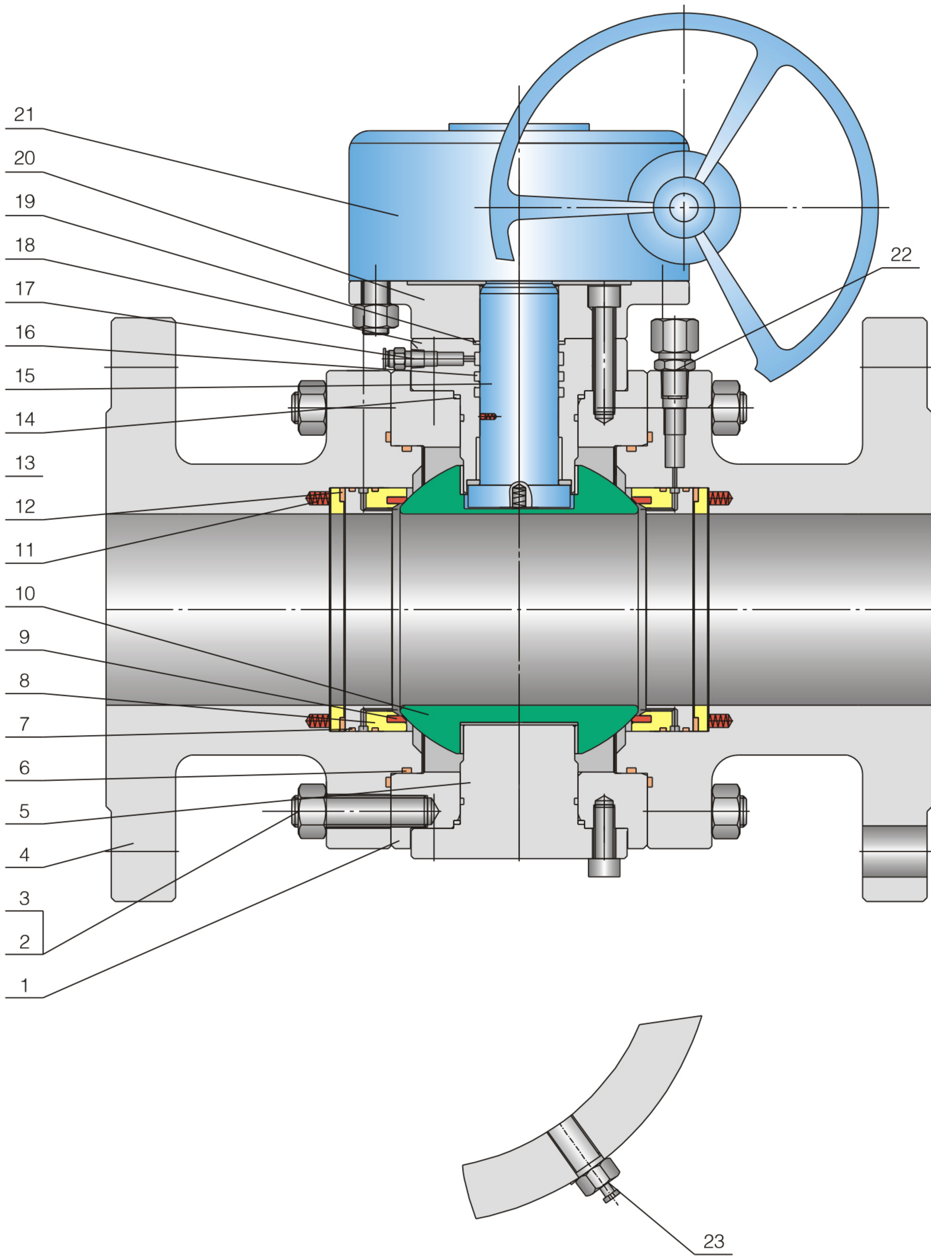
主要结构图形 Major Features
