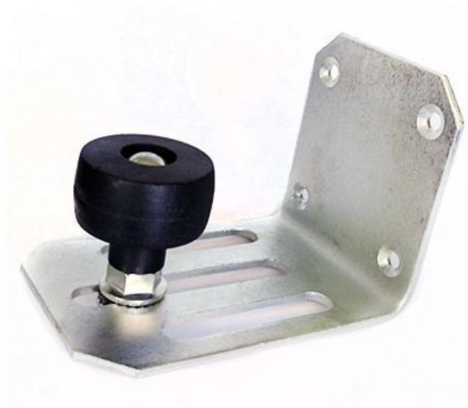
Item No.: M00073 Size: 5"*6"*6mm Material: Steel Finished: Zinc plated
