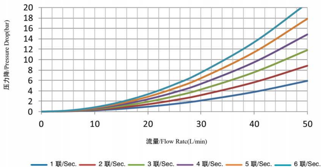
Pressure Drop at neutral position (P to T) 中位时, 进口口到油箱的压力降 (P to T)
