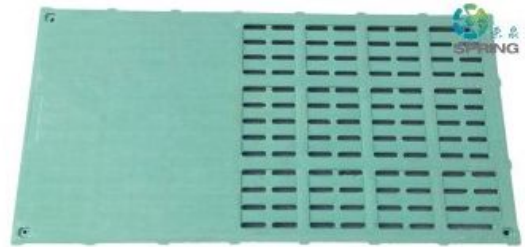
Name: BMC Slat Floor For Sow(1.2M) Type: RQLF007-1200*600*35 Gap: 11mm
