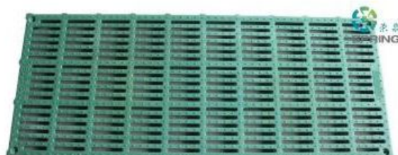
Name:BMC Slat Floor For Nursery Pig Type:RQBY004-1500*600*35 Gap:14mm
