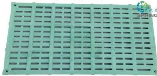
Name: BMC Slat Floor For Sow(1.2M) Type: RQLF006-1200*600*35 Gap: 11mm
