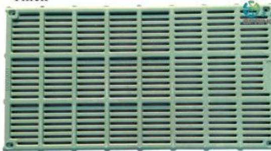
Name: BMC Slat Floor For Sow (Thick) Type: RQLF001C-1100*600*38 (Model C) Gap: 11mm
