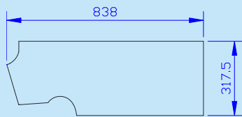
NS-9264下模 Lower mould
