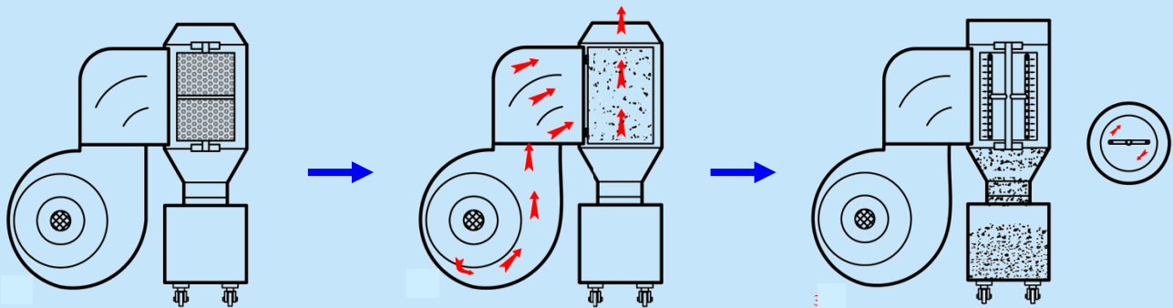
自動環保除塵系統工作原理圖 Work principle of environment-friendly automatic de-dusting & filtering system
