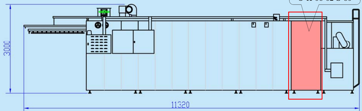
NS-395E-50 標準機型+運輸帶焗爐預熱系統-蒸汽 Standard + Steam Preheating System for Conveyer Belt Oven
