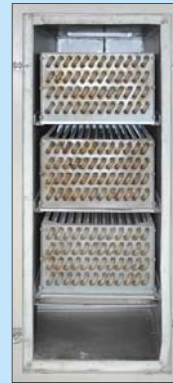
O-K-06-02-S-80 運輸帶焗爐預熱系統-蒸汽 (僅適用於NS-395E-50) Steam Preheating System for Conveyor Belt Oven (for NS-395E-50 only)
