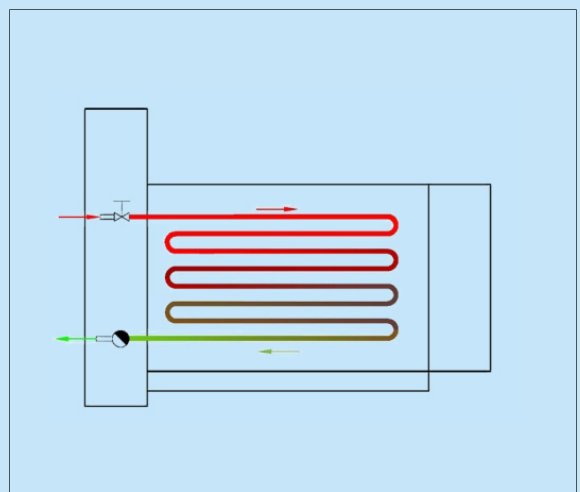
蒸汽間接加溫示意圖(NS-2713系列) Indirect steam heating diagram (NS-2713 series)
