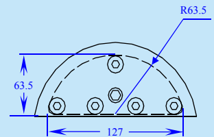
下模尺寸簡圖 Dimensions Diagram of the Lower Mould
