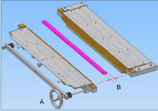
筒模夾具系統，可快捷更換筒模 A:旋轉手柄 B:前筒模寬度 Clamping system of placket folding mould for quick and convenient mould changing A. Hand wheel B. Shirt placket mould width
