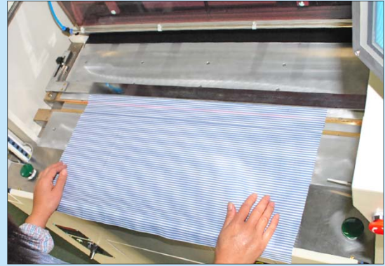
鐳射光線輔助對齊，方便對格對條 Laser light assists users to check and stripe matching
