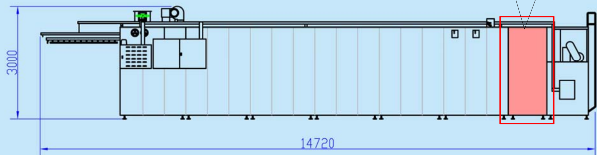
NS-395E-80 標準機型+運輸帶焗爐預熱系統-蒸汽 Standard + Steam Preheating System for Conveyor Belt Oven
