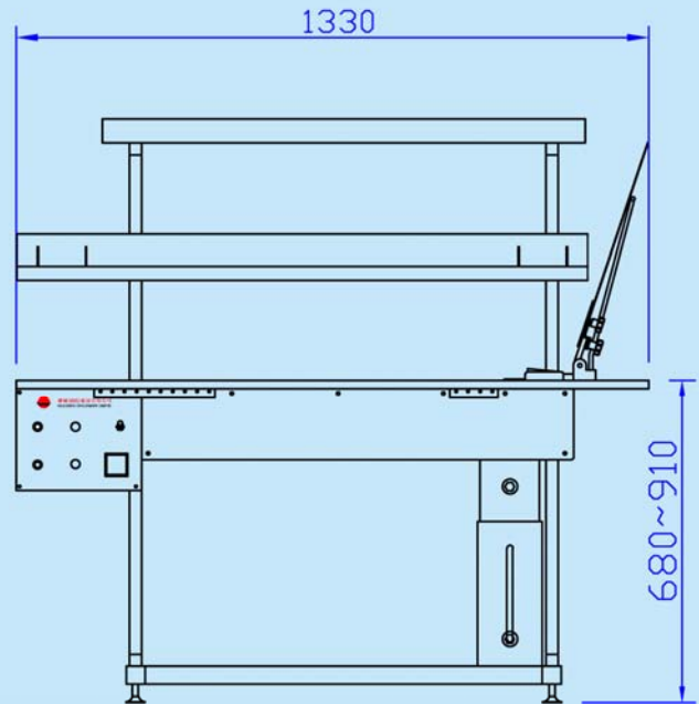
可根據習慣更換操作方向 Alternative Layout to suit operating habit
