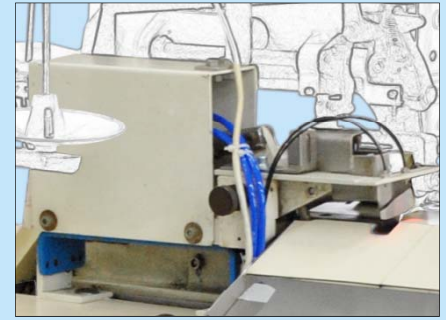
電眼感應裝置連切刀 Electric eye sensing device with cutter
