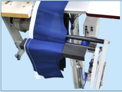
夾布桿夾布 Fabric clamping
