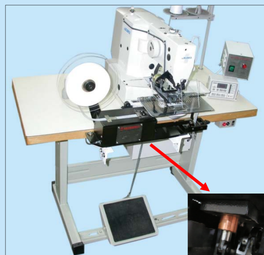
安裝在縫紉機上 Installed on a sewing machine
