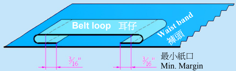
耳仔成品示意圖 Schematic Diagram of finished belt loop
