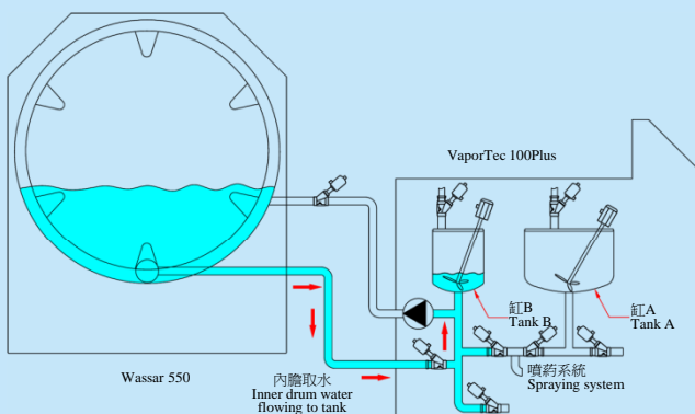
內膽取水示意圖 Diagram of inner drum water flowing to tank
