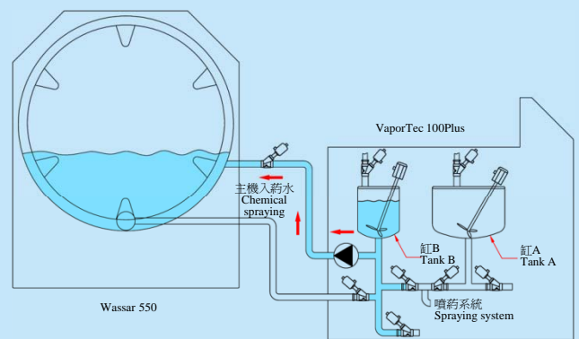
藥水噴入內膽示意圖 Diagram of chemical spraying to inner drum
