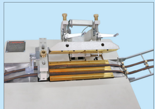
1/2 "立體耳仔下模 1/2 " 3-D belt-loop lower mould
