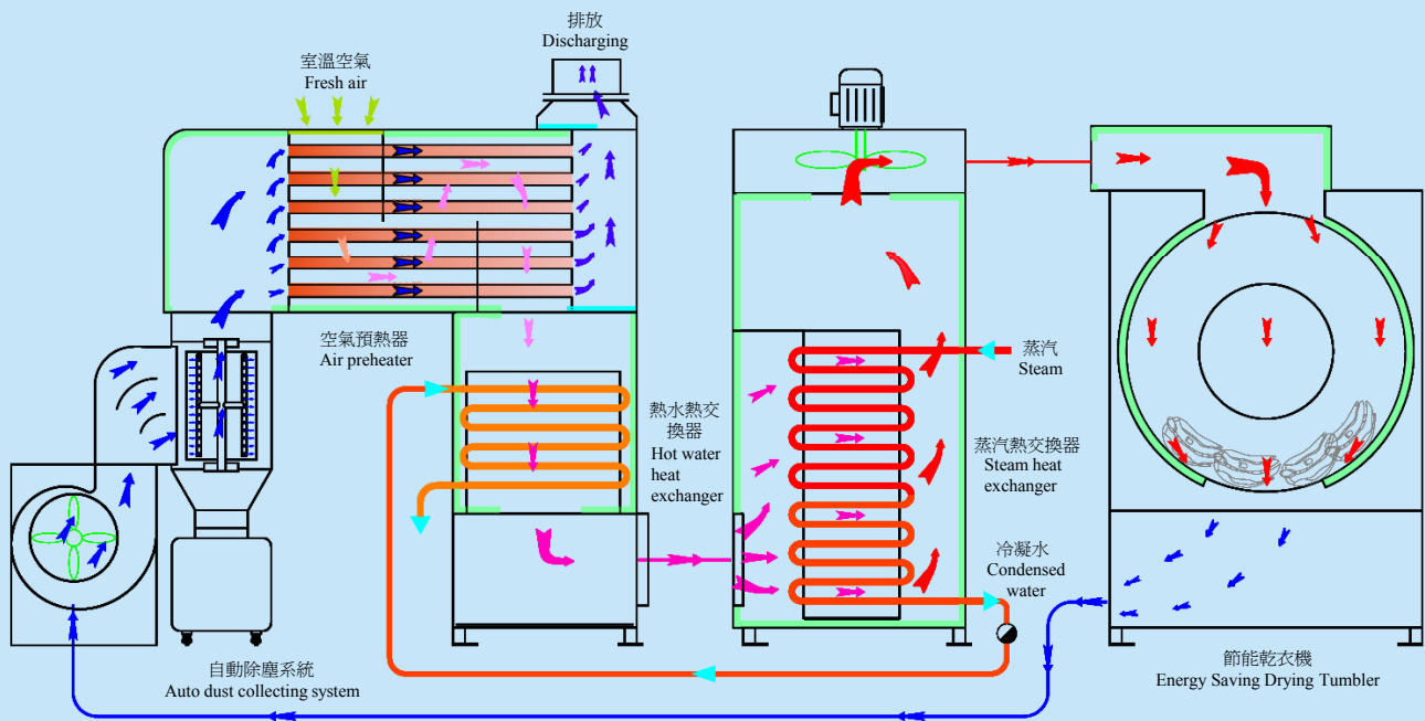
乾衣機工作原理圖 Working principle diagram of drying tumbler
