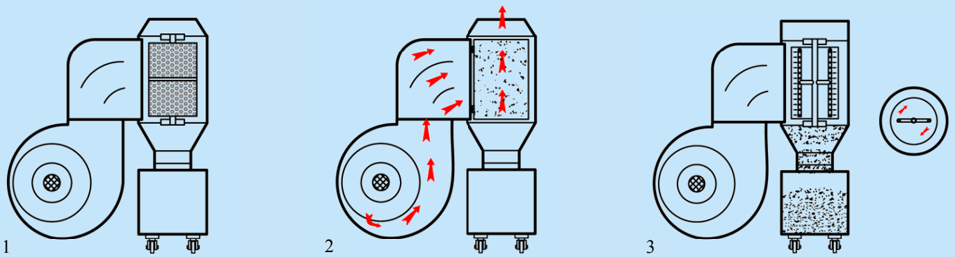
自動環保除塵系統工作原理 Working principle of environment-friendly automatic de-dusting & filtering system
