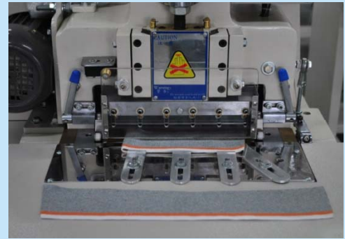
修領腳操作 Trimming operation
