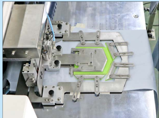
4.折袋完成，準備送入車縫工序 Pocket folding finished, ready for being conveyed to sewing station
