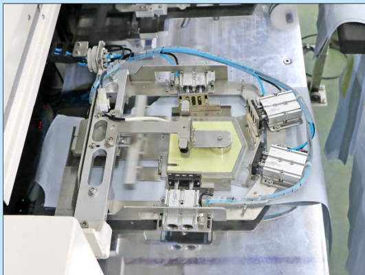
3.機器自動折袋 Automatic pocket folding by machine
