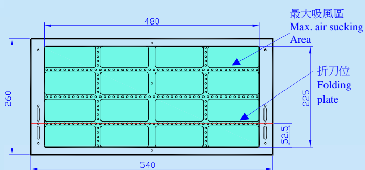
下模底座尺寸示意圖 Dimensions Diagram of Lower Mould Base
