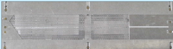
中東長袍半胸筒模 Placket Mould of Arabian Robe
