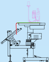
1.裁片車縫中 Sewing in process
