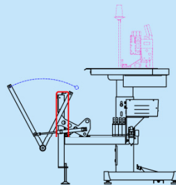
3.撥布桿撥布 Pushing fabric aside
