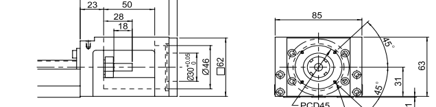
Motor Adaptor Flange F3
