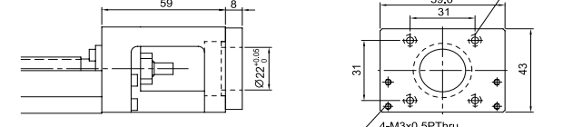
Motor Housing H1
