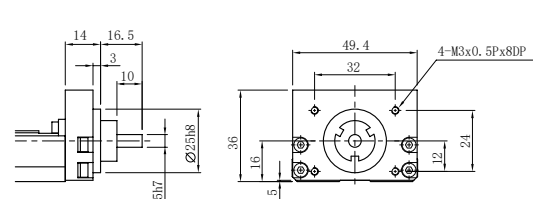
Motor Housing H0
