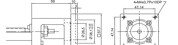
Motor Adaptor Flange F5
