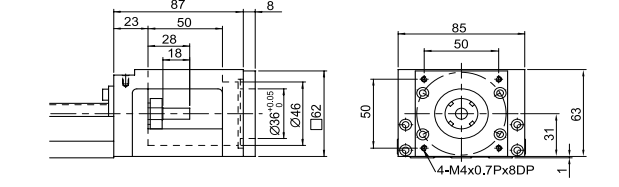
Motor Adaptor Flange F6
