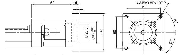
Motor Adaptor Flange F4
