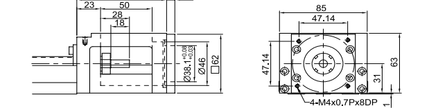
Motor Housing H0
