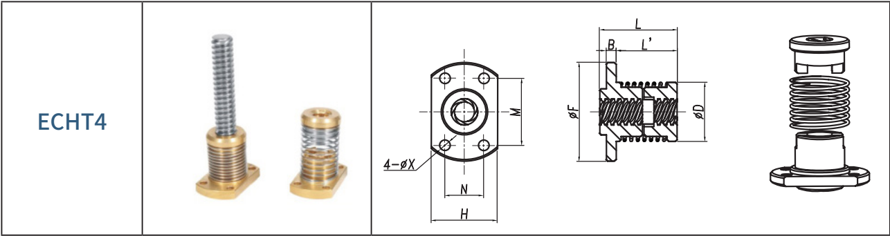
Anti-backlash nut | ECHT4 series
