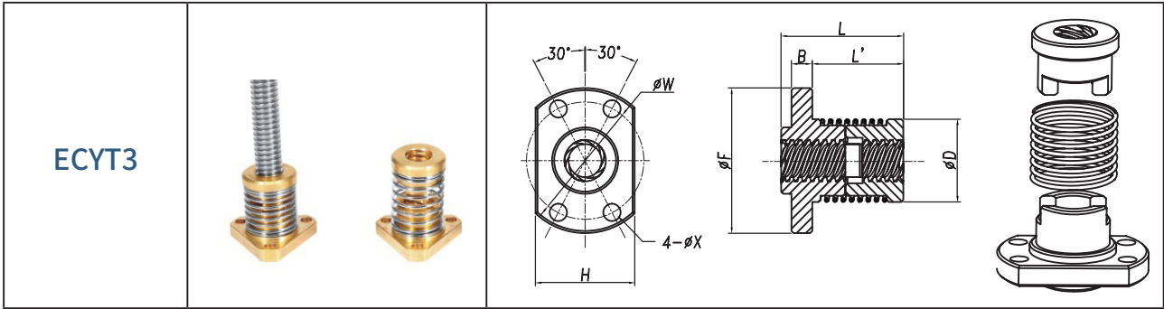
Anti-backlash nut | ECYT3 series
