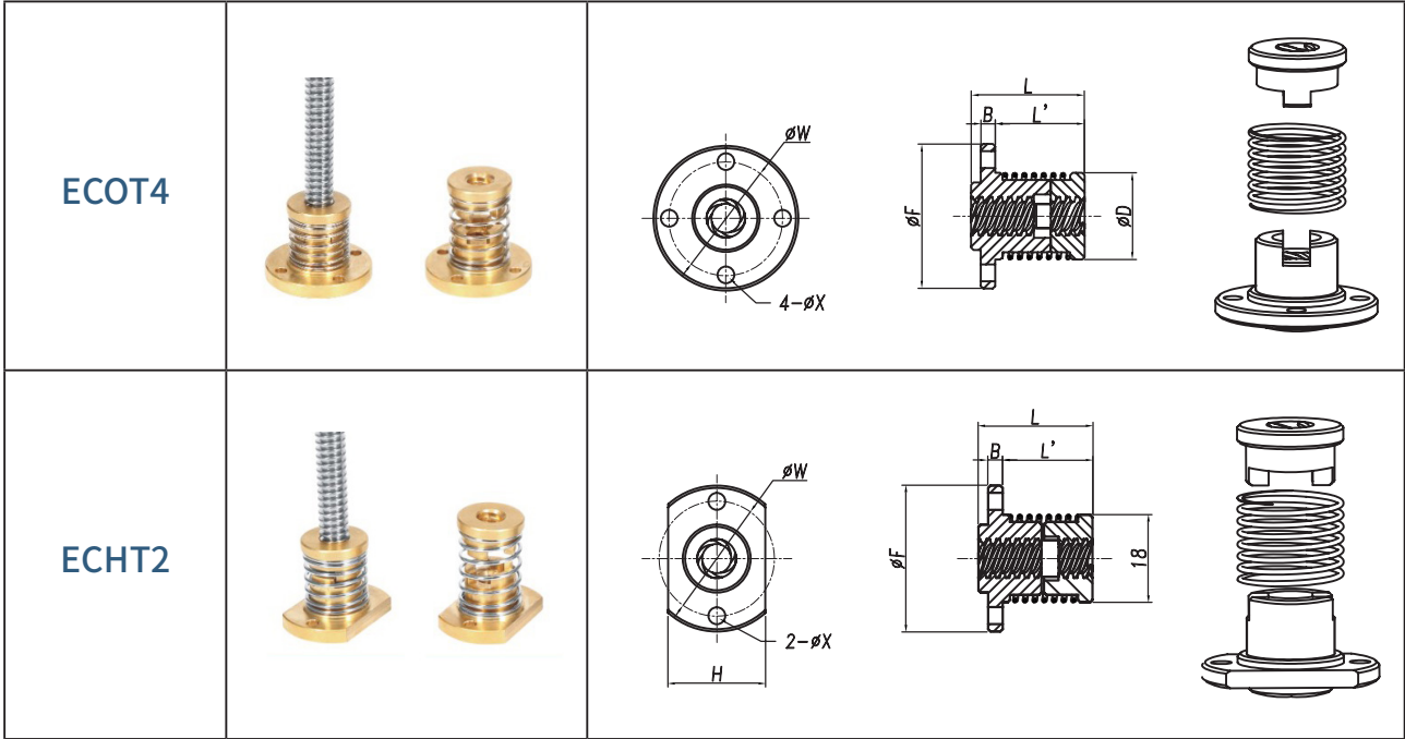
Anti-backlash nut structure | ECOT4/ECHT2 series
