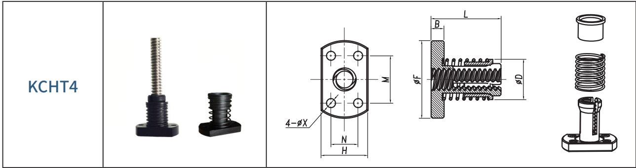
Anti-backlash nut | KCHT4 series
