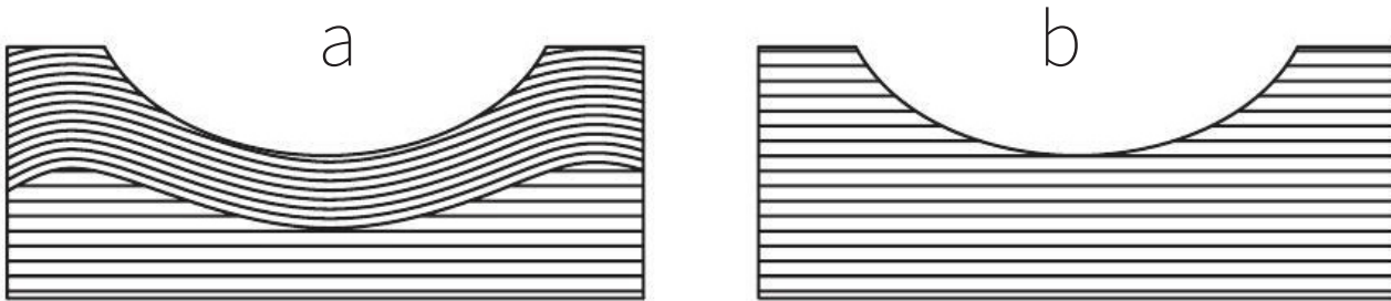
Rolling process
