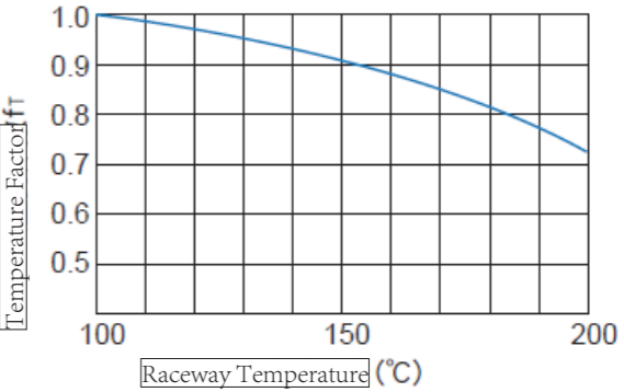
Fig 2.2.2 Temperature Factor ( fT)
